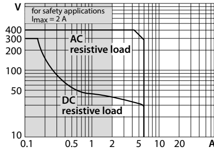
Fig. 5: Load Curve
